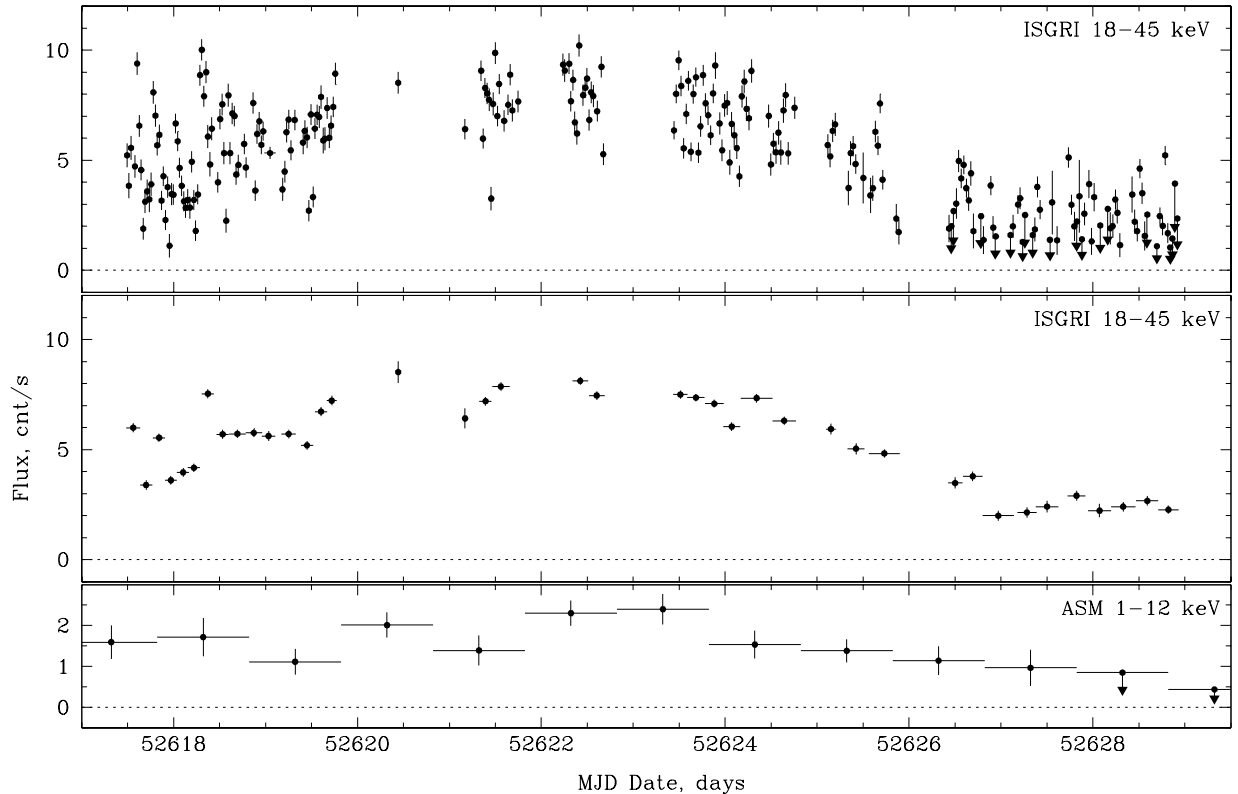
Fig. 2. Light curves of EXO 2030+375 in 18–45 keV (top and middle) and 1–12 keV energy bands. Data points of top pannel correspond to observations of each particular “Science Window” and count rate was extracted directly from source reconstructed spectra. Source flux below 2\sigma detection level replaced by 2\sigma upper limits. Data averaged over 1–6 “Science Windows” are shown in middle panel. Light curve obtained bt RXTE All Sky Monitor (ASM) is shown in bottom for comparison. Correlation of source fluxes between in IBIS/ISGRI and RXTE/ASM observations is apparent.
