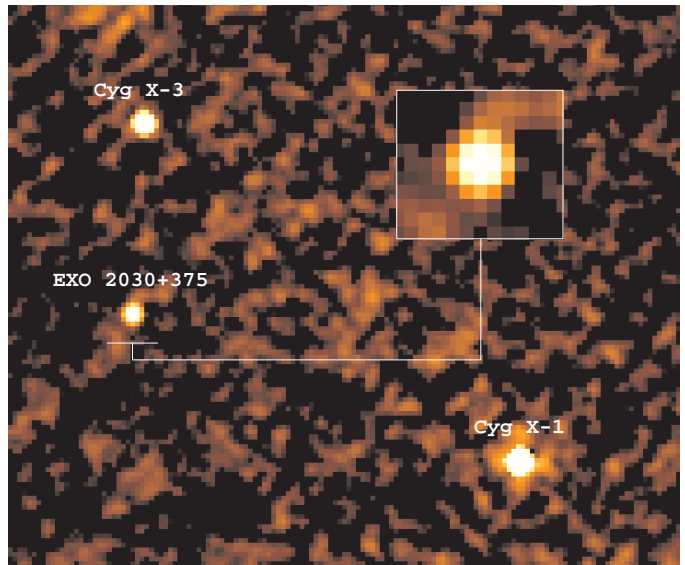
Fig. 1. Image of Cygnus region in 18–45 keV energy band averaged over 142 ksec of observations during 19th revolution. Image size is \sim 9.7^\circ \times 11.7^\circ , size of zoomed region of EXO 2030+375 centered at 20^{\text{h}}32^{\text{m}}19.8^{\text{s}} + 37^\circ 38^{\text{m}}15.5^{\text{s}} is 0.9^\circ \times 0.9^\circ . Sources were detected with following significance of 1300\sigma , 210\sigma and 90\sigma for Cyg X-1, Cyg X-3 and EXO 2030+375, respectively. Squared root scale was used for color representation.
